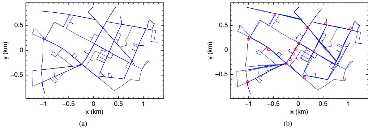
Fig. 5: Results of solving a simulated pose-graph representing driving around Cambridge, Massachusetts for approx. 75 km using: a) a location database containing all 712 street intersections, and b) a dramatically reduced database of only 15 pre-selected intersections (0.5% of the full database of 3,375 poses). The true positions of the selected database entries are shown in red. It is clear that, due to the high quality of the 15 selected locations, the topology of the map is still captured.
