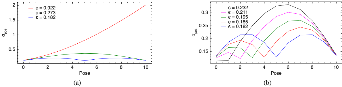
Fig. 2: Effects on error covariance for a sequence of 11 poses due to: (a) adding additional loop-closures, and (b) changing their spatial distribution. The average pose uncertainty \epsilon (7b), which we aim to minimize, is provided in the legend. Note that in these plots, we have assumed that loop-closure constraints are added to already-well-estimated poses in the map, thus modeling them as location priors.
