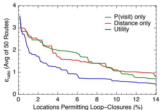
Fig. 9: Comparison of the effects of the two objectives that form the “location utility” on pose smoothing covariance. The green line determines location utility using only visit probability ( v ), the red line uses only distance ( d ), and the blue line uses an equal combination of the two terms. Note that all three approaches are initialized using the location with maximum P(\text{visit}) for |D| = 1 .
