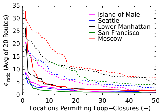
Fig. 8: Comparison of average pose uncertainty using locations selected by our method (solid lines) vs. randomly (dashed lines) for a vehicle navigating in five cities.
