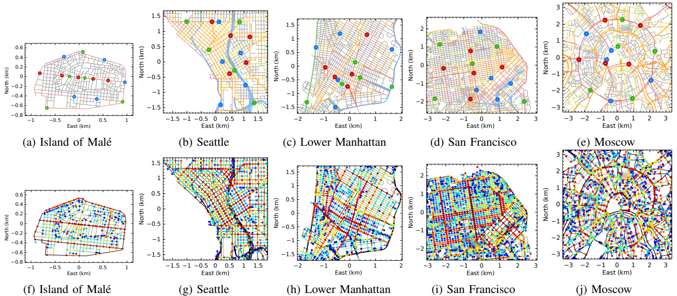
Fig. 7: The best 1-5 (red), 6-10 (green), and 11-15 (blue) street intersections (top) and all street intersections sorted based on loop-closure utility (bottom) for five major cities around the world, with maximum database sizes ranging from 535 to 2811 locations, increasing from left to right. In all cases, our algorithm favors both locations on major highways and locations spatially distributed evenly between them.
