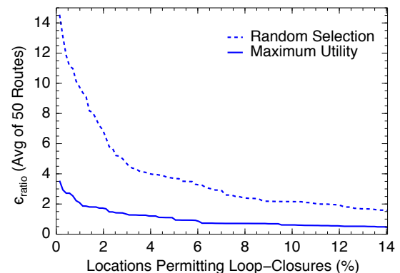
Fig. 6: Comparison of average pose uncertainty when using location databases selected using our method vs. randomly for a vehicle navigating in Cambridge, Massachusetts.
