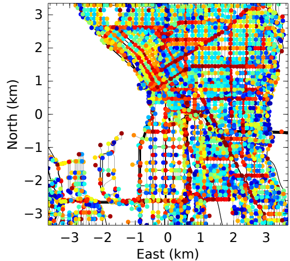
Fig. 1: Street intersections in Seattle, Washington , which are sorted based on their location utility as proposed in this paper. Such utility is a combination of the probability that a location is visited on any point-to-point shortest-time route through the environment and a spatial distribution term (see Section III), and is used to select a reduced location database for a storage/computation-constrained SLAM system, seeking to minimize map uncertainty without a priori knowledge of the vehicle trajectory. Note that in this graph, dark red denotes the maximum utility while dark blue is the minimum.
