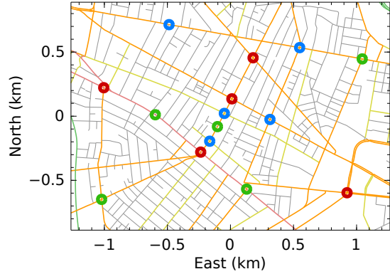
Fig. 4: Best 5 (red), 10 (red + green), and 15 (red + green + blue) locations selected for a minimal database for a region of Cambridge, Massachusetts.
