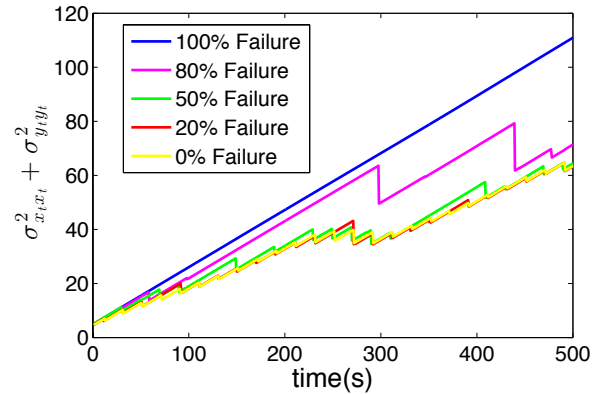
Fig. 6. The instantaneous (filtered) location uncertainty of AUV 1 using the proposed method for different dropout rates.
