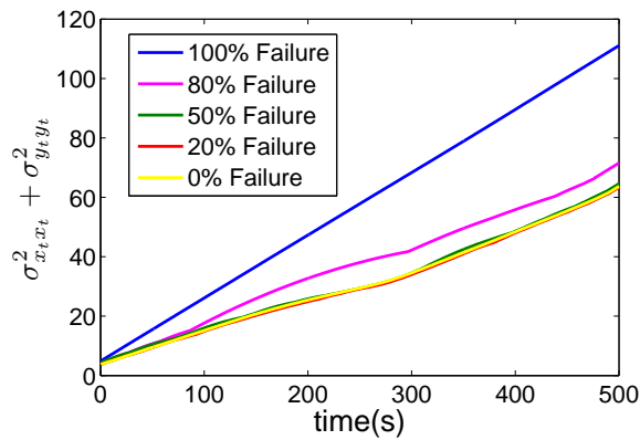
Fig. 8. The location uncertainty of the smoothed estimate at time t = 500s of AUV 1 using the proposed method for different dropout rates.
